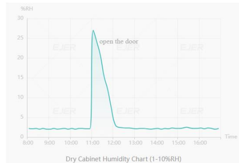
With rapid dehumidification module
