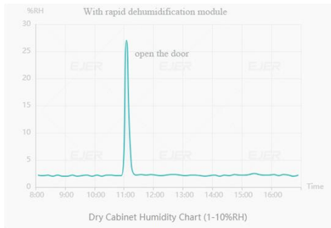
Standard dry cabinet humidity chart (1–10%RH)
